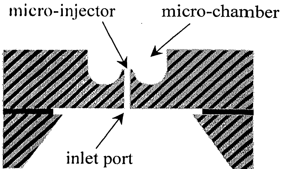
Fig. 2. A representative view of a single injector
